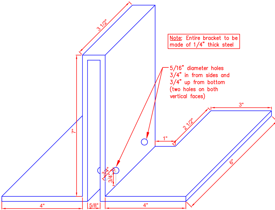
Custom Bracket 3D View
